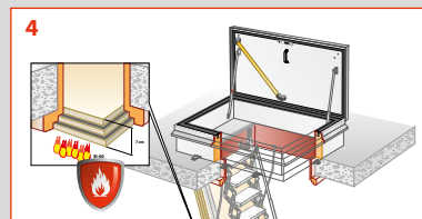
» RHT7014 + EI-60 Fire rating class EI-60
