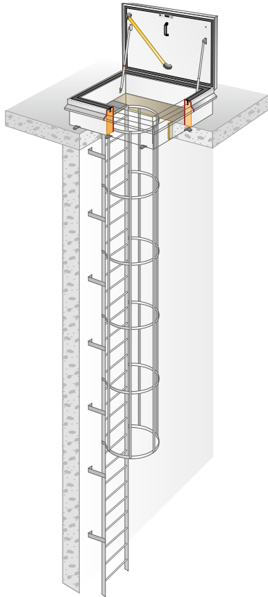
» Vertical fixed ladder with safety cage
