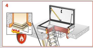
» RHT7014 + EI-60 Fire rating class EI-60
